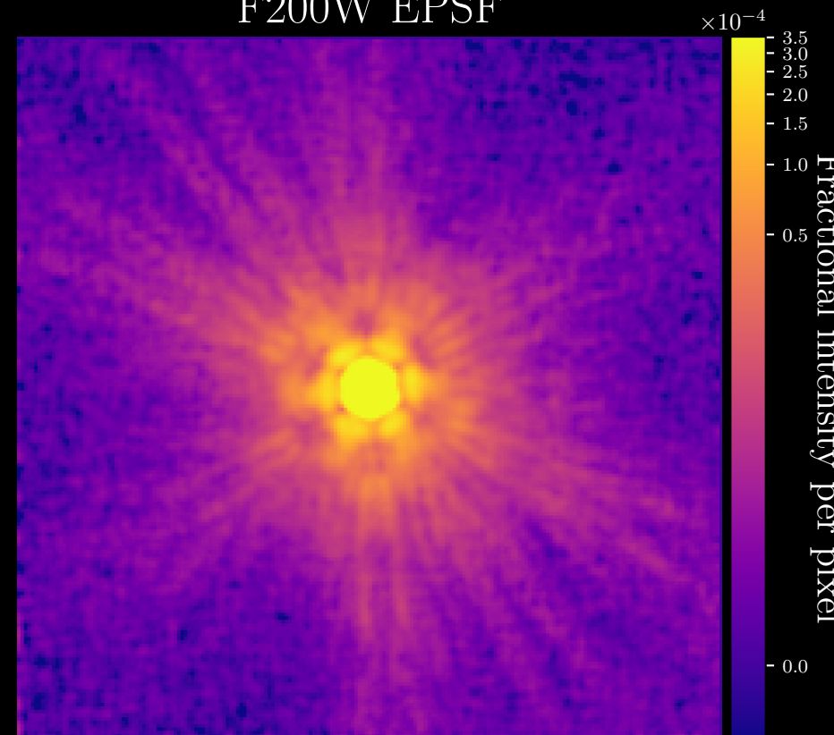
F200W EPSF
