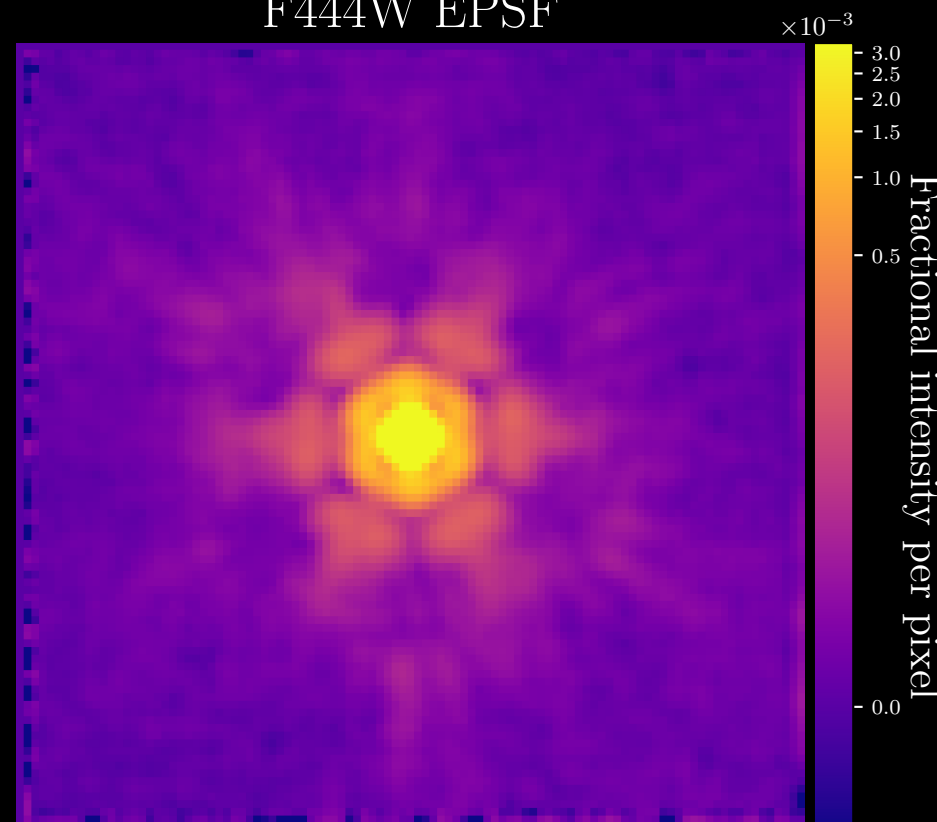
F444W EPSF
