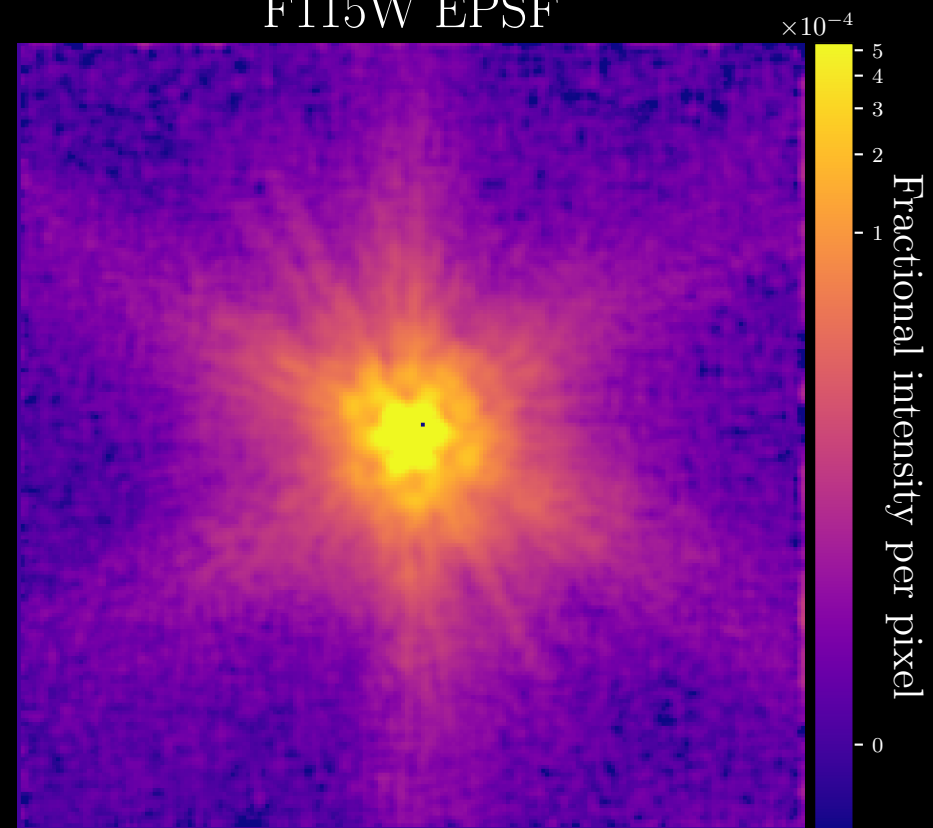
F115W EPSF
