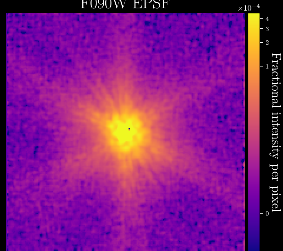
F090W EPSF
