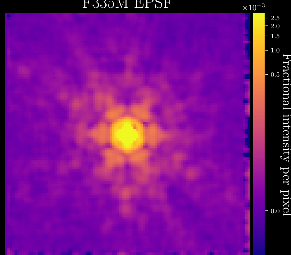
F335M EPSF
