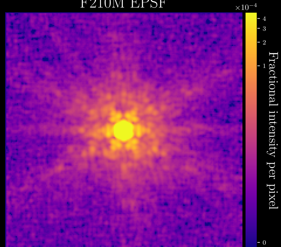
F210M EPSF
