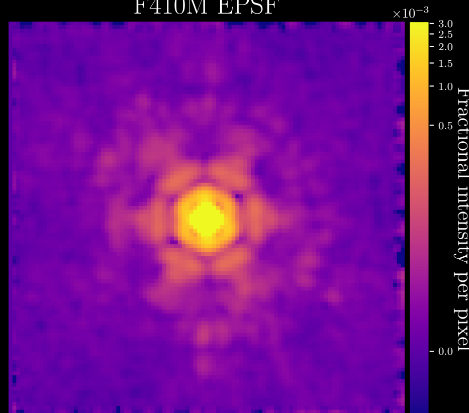
F410M EPSF
