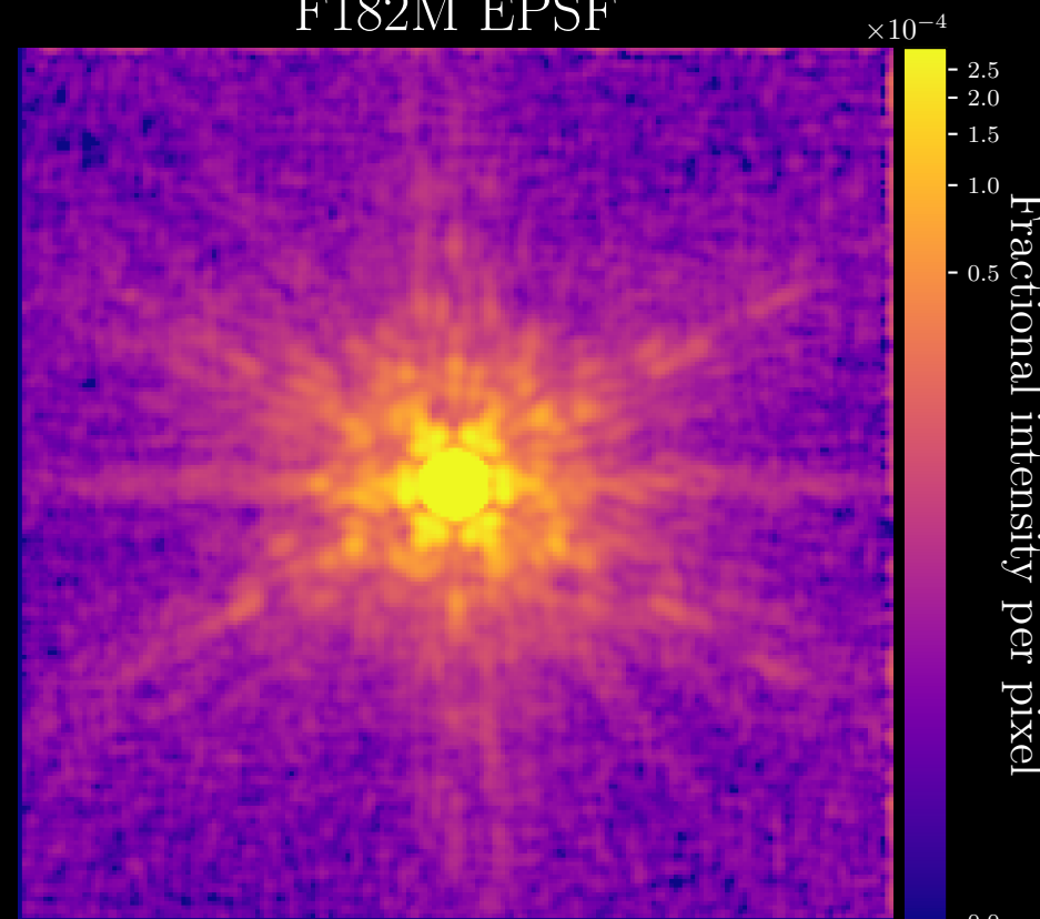
F182M EPSF
