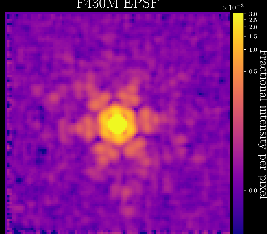
F430M EPSF
