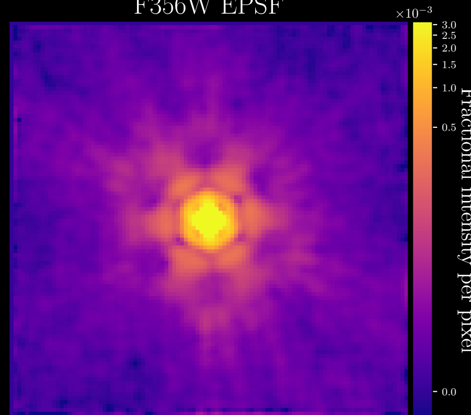
F356W EPSF
