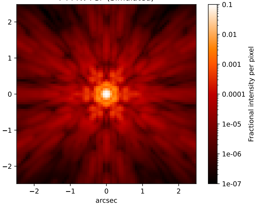
F444W PSF (Simulated)
