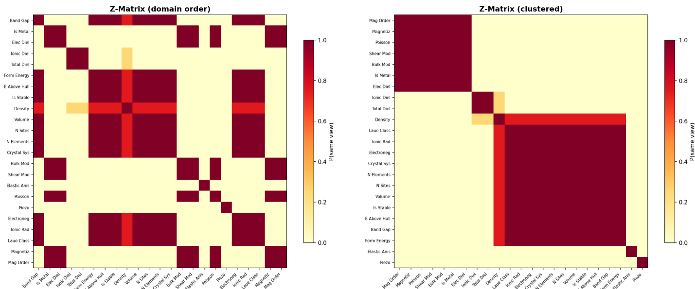
Figure 2: Z-matrix (dependence probability). Clear block structure: structural/thermodynamic (View 0), electronic/mechanical (View 1), and ionic dielectric pair (View 2).
