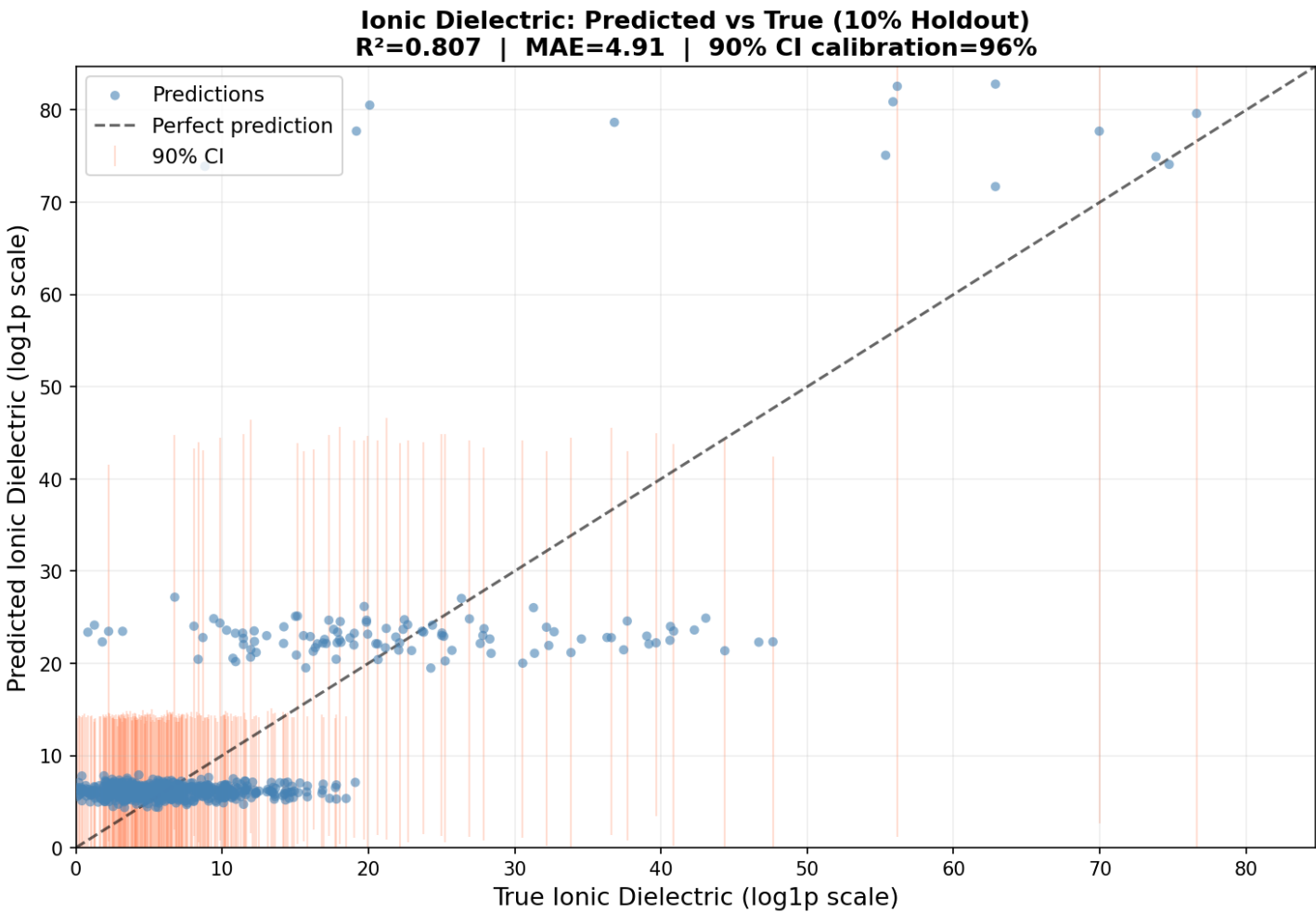
Figure 3: Ionic dielectric predicted vs. true (holdout). R^2=0.81 with 90% credible intervals. The model achieves 88% of Random Forest accuracy while also providing structure discovery and calibrated uncertainty.
