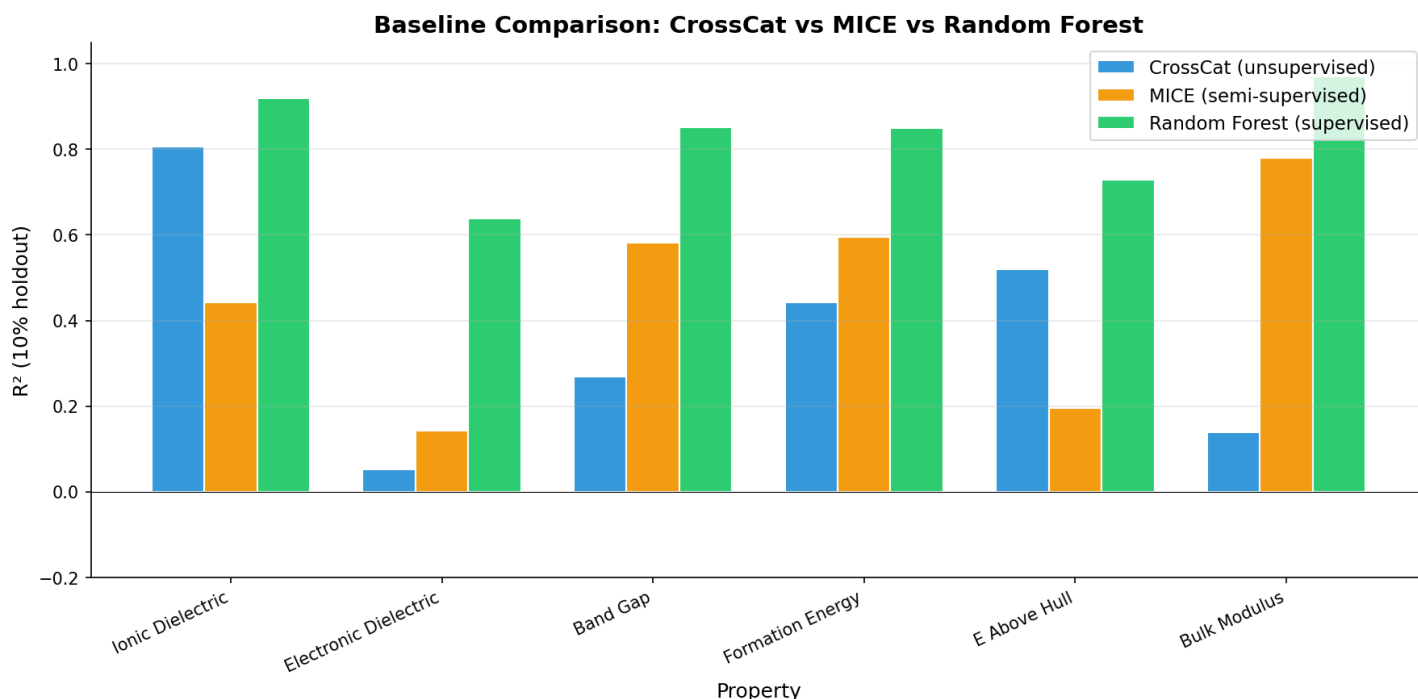
Figure 7: R^2 comparison on 10% holdout. RF wins on raw accuracy (green) but requires per-target training and provides no uncertainty. CrossCat (blue) is a general-purpose model that also discovers structure and quantifies uncertainty.
