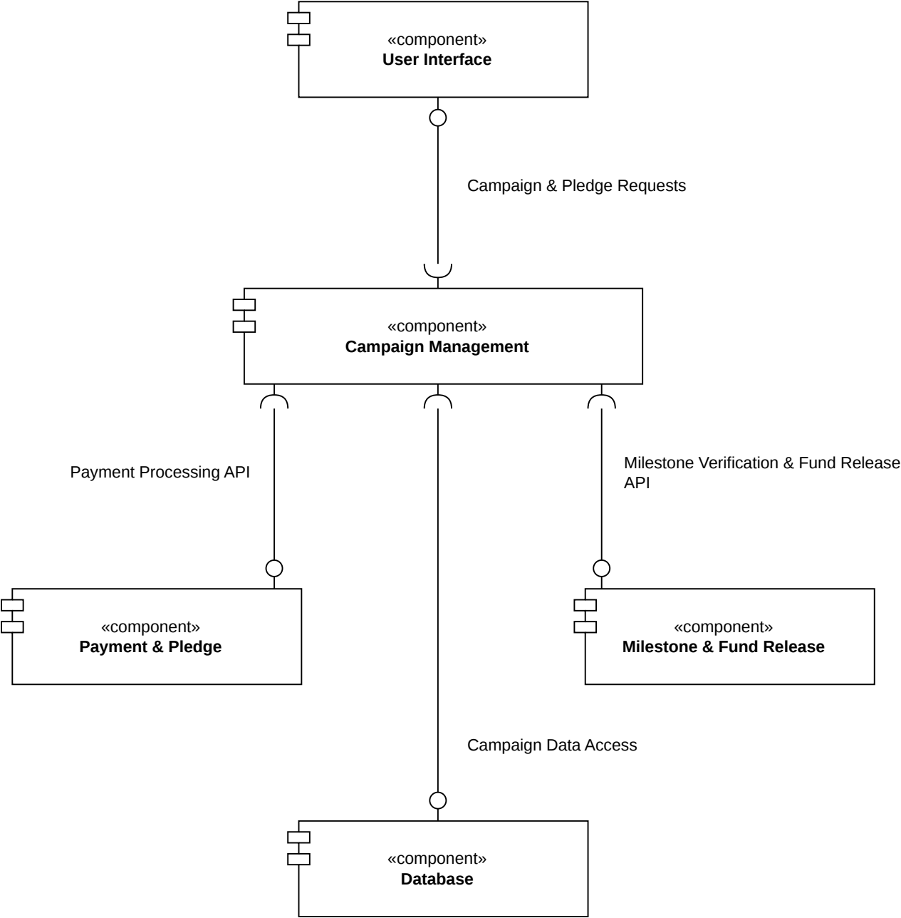
UML Component Diagram — Layered Architecture
