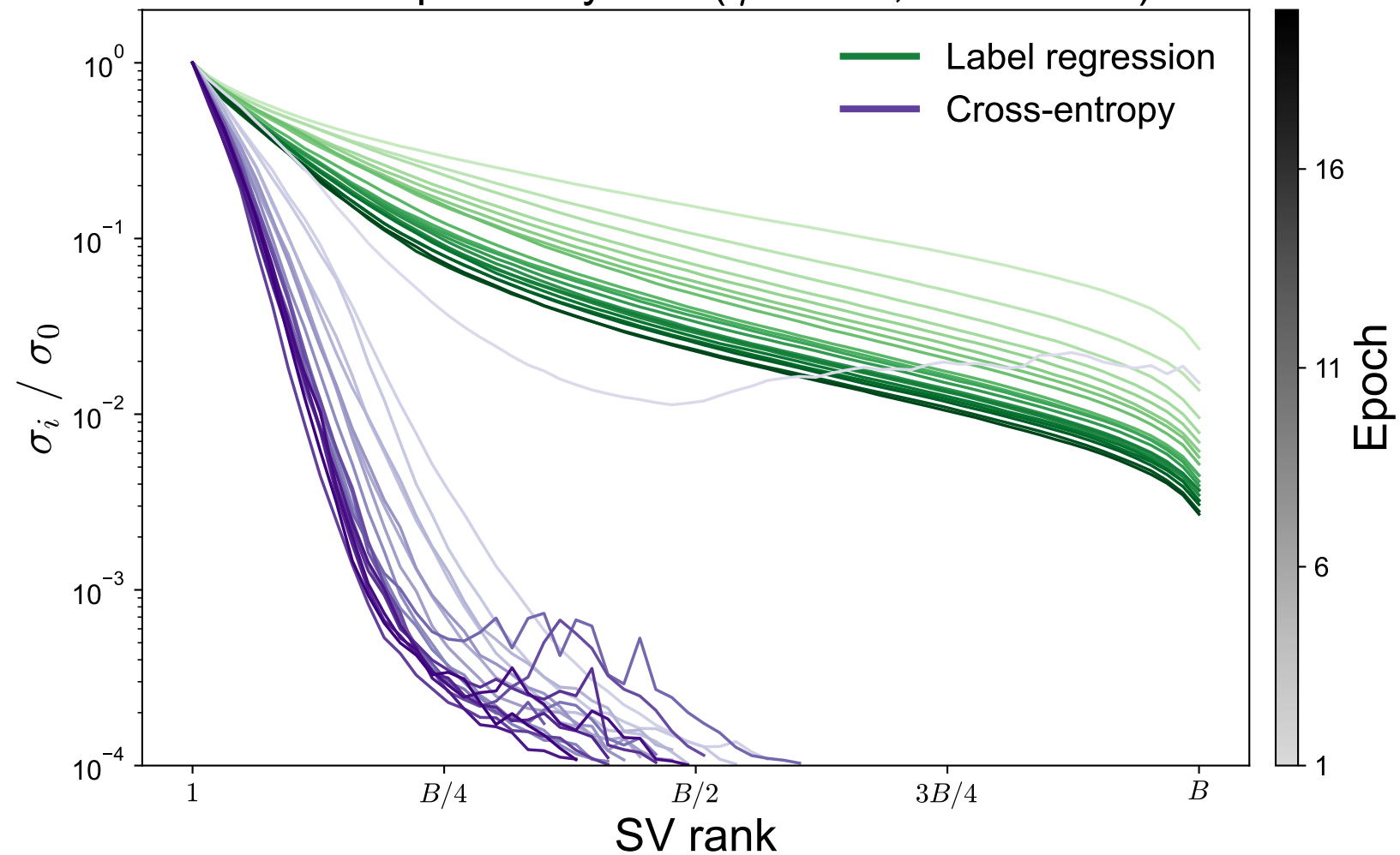
MNIST spectra by loss ( \eta = 10^{-1} , \text{rtol} = 10^{-4} )
