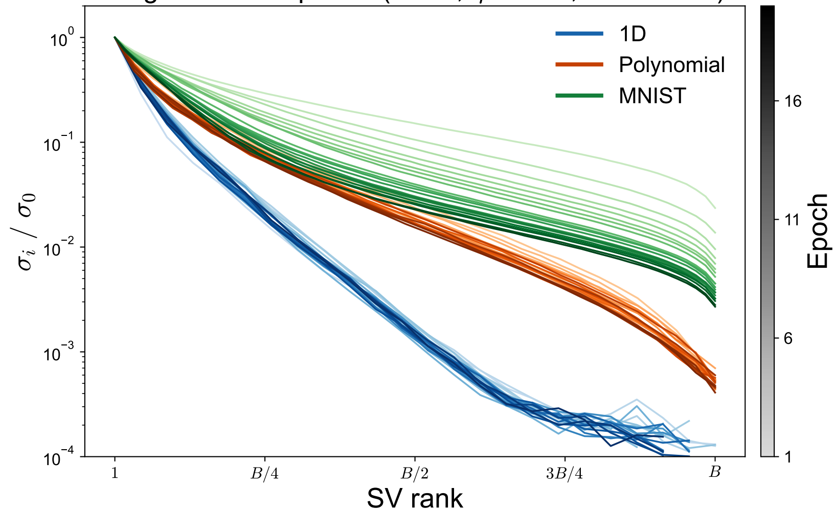
Singular value spectra ( k = B , \eta = 10^{-1} , \text{rtol} = 10^{-4} )
