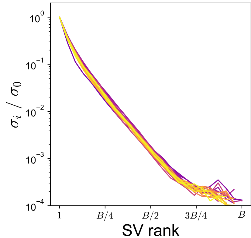
1D
