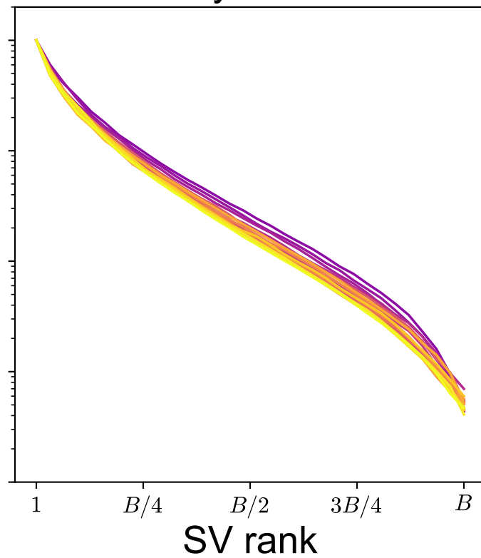
Polynomial
