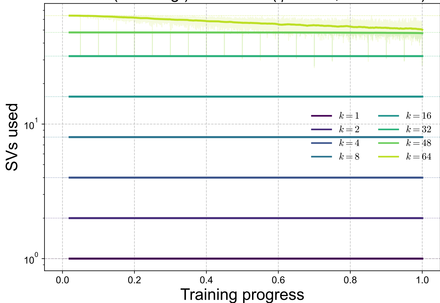
MNIST (label reg.): SVs used ( \eta = 10^{-1} , \text{rtol} = 10^{-2} )
