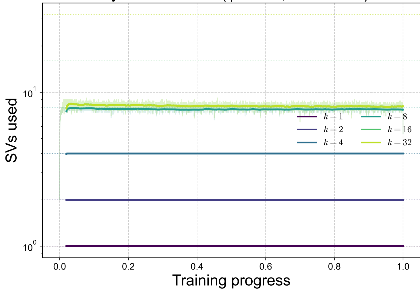
Toy 1D: SVs used ( \eta = 10^{-1} , \text{rtol} = 10^{-2} )
