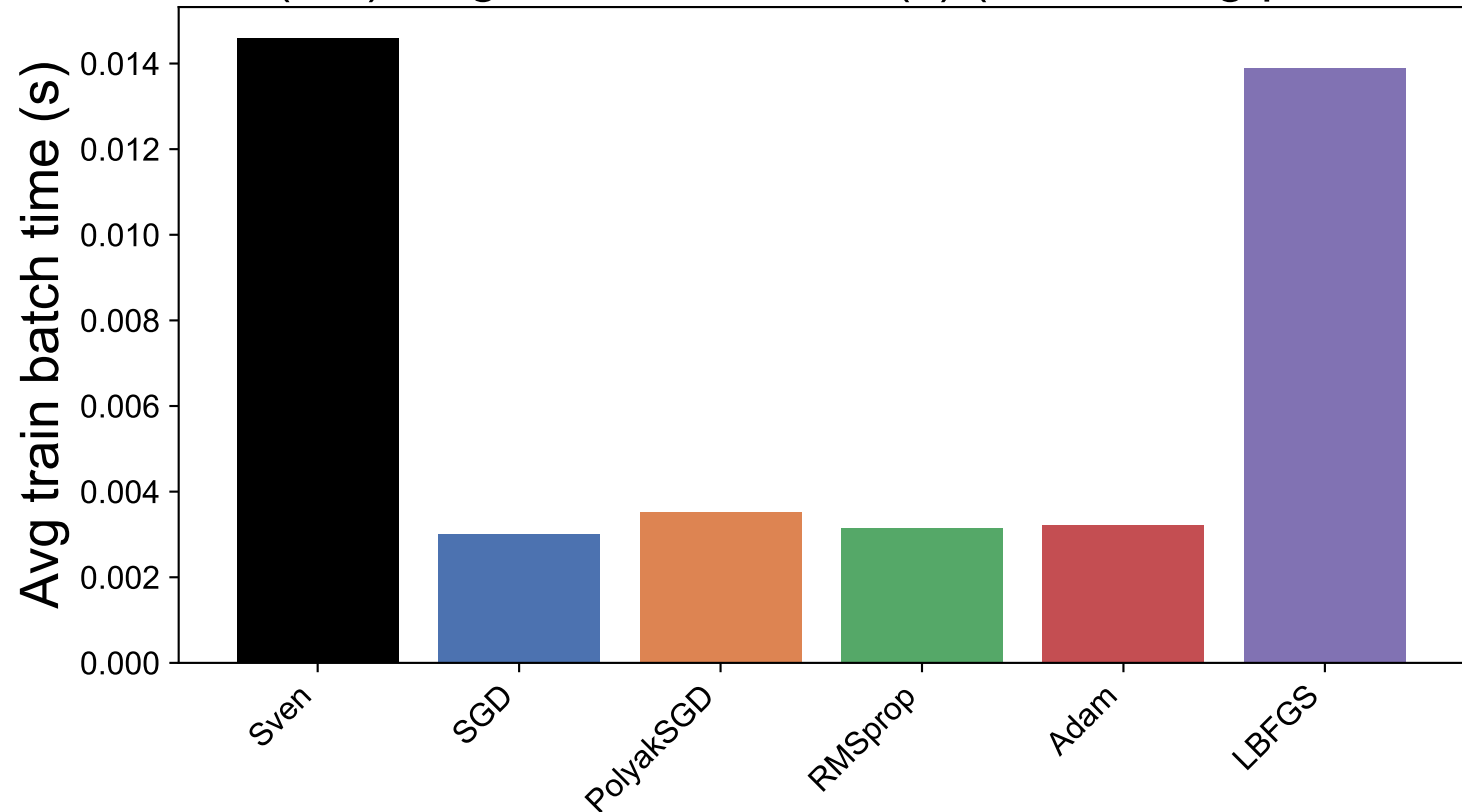
MNIST (CE): avg train batch time (s) (best config per method)
