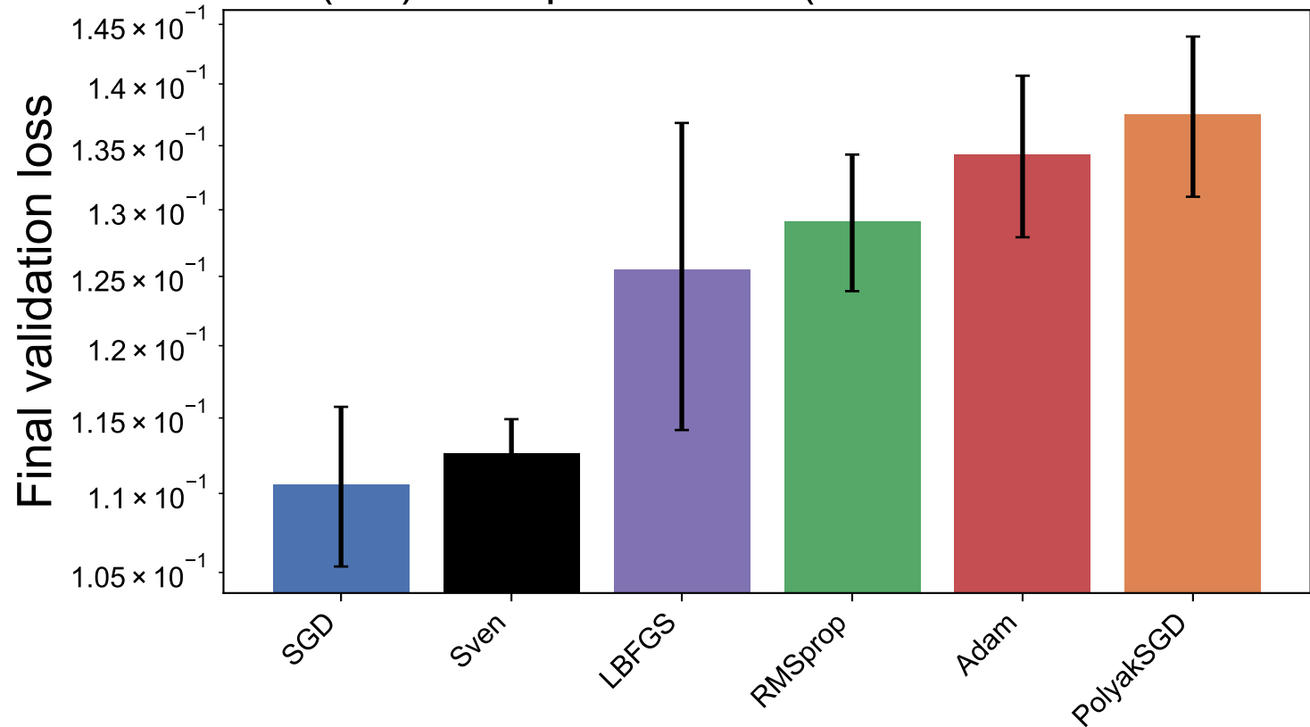
MNIST (CE): best per method (mean \pm s.d. over 5 seeds)
