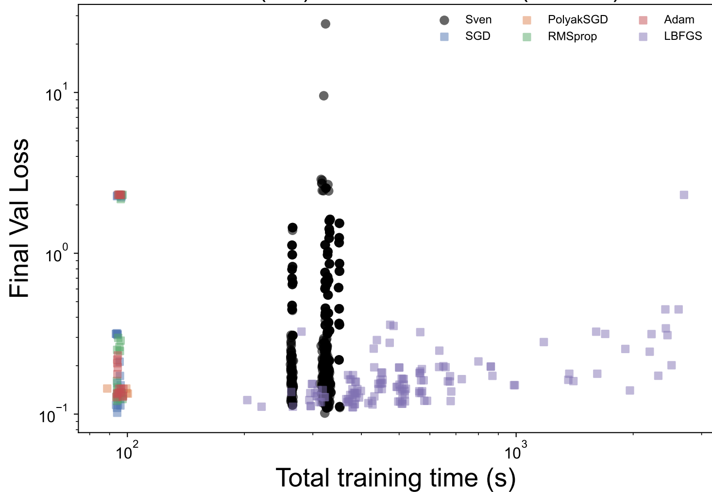
MNIST (CE): loss vs wall time (all runs)
