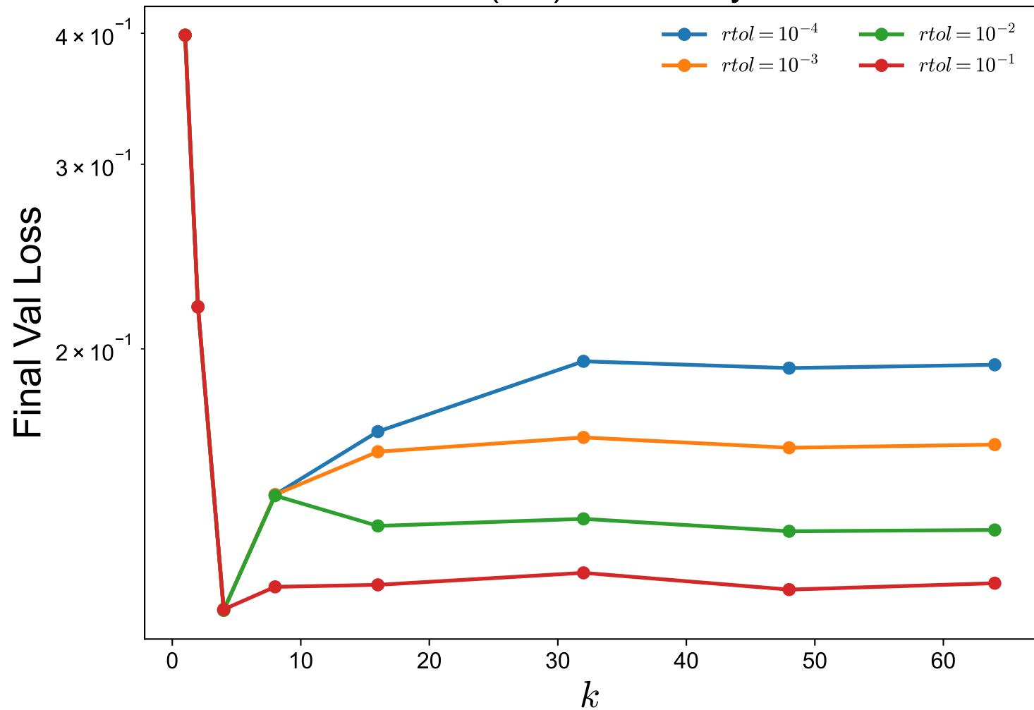
MNIST (CE): sensitivity to k
