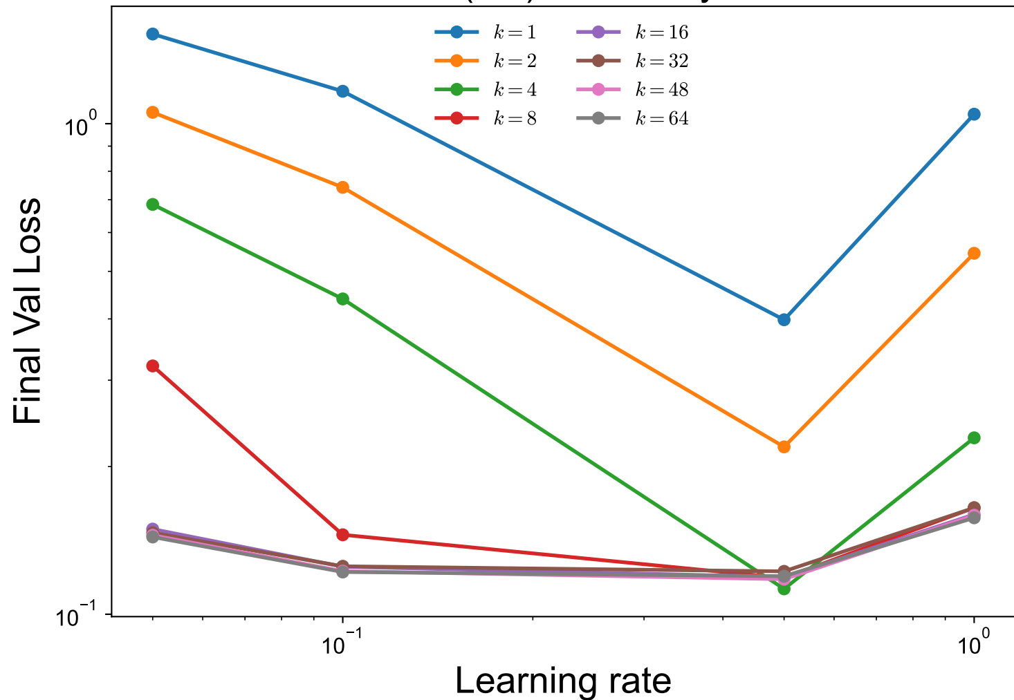
MNIST (CE): sensitivity to lr
