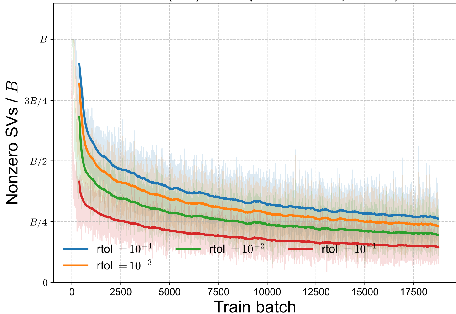
MNIST (CE): rank ( k = B = 64 , \eta = 0.05 )
