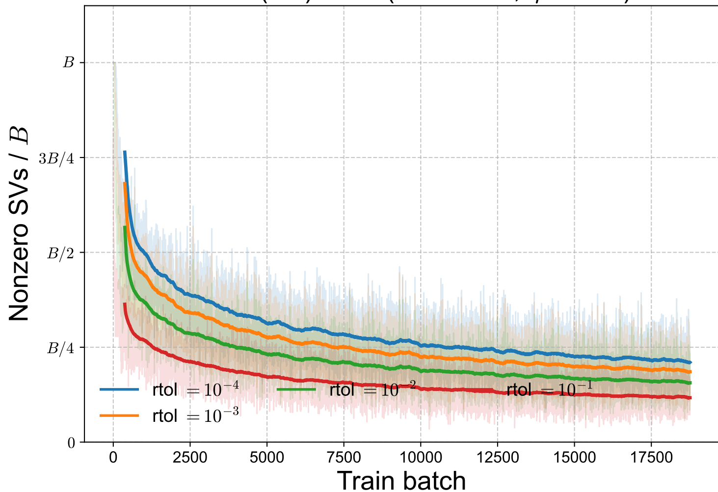
MNIST (CE): rank ( k = B = 64 , \eta = 10^{-1} )
