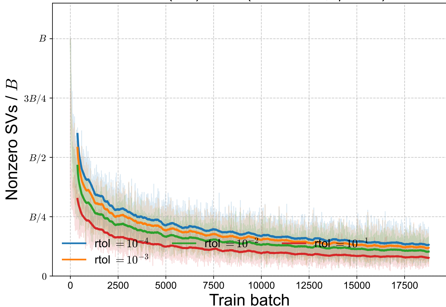
MNIST (CE): rank ( k = B = 64 , \eta = 0.5 )
