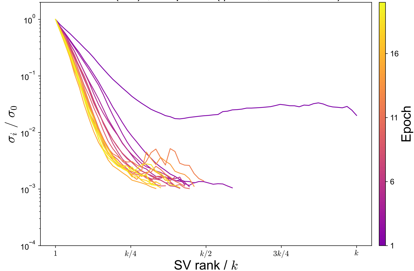
MNIST (CE): SV spectra ( \eta = 10^{-1} , \text{rtol} = 10^{-3} )
