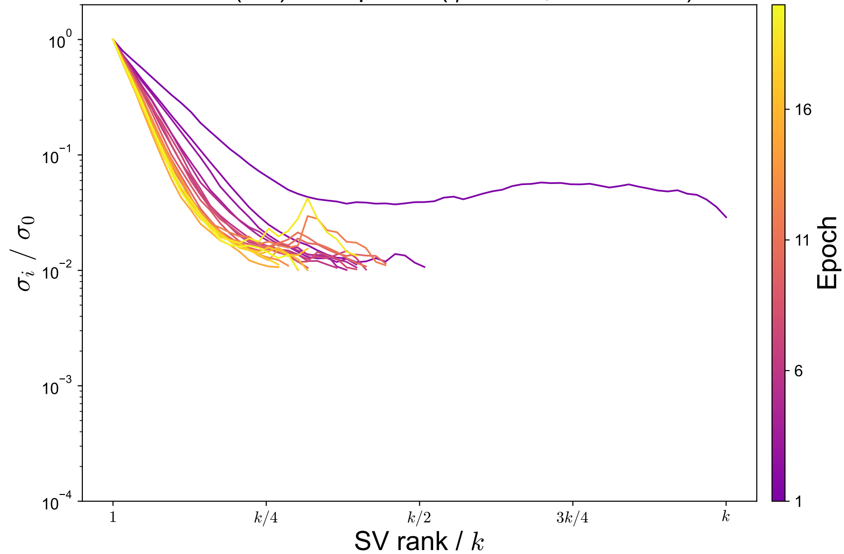
MNIST (CE): SV spectra ( \eta = 10^{-1} , \text{rtol} = 10^{-2} )
