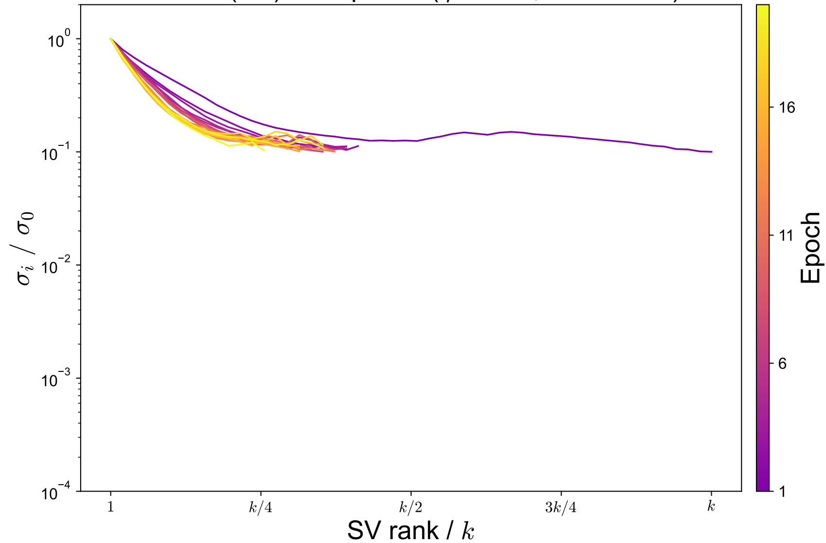
MNIST (CE): SV spectra ( \eta = 10^{-1} , \text{rtol} = 10^{-1} )
