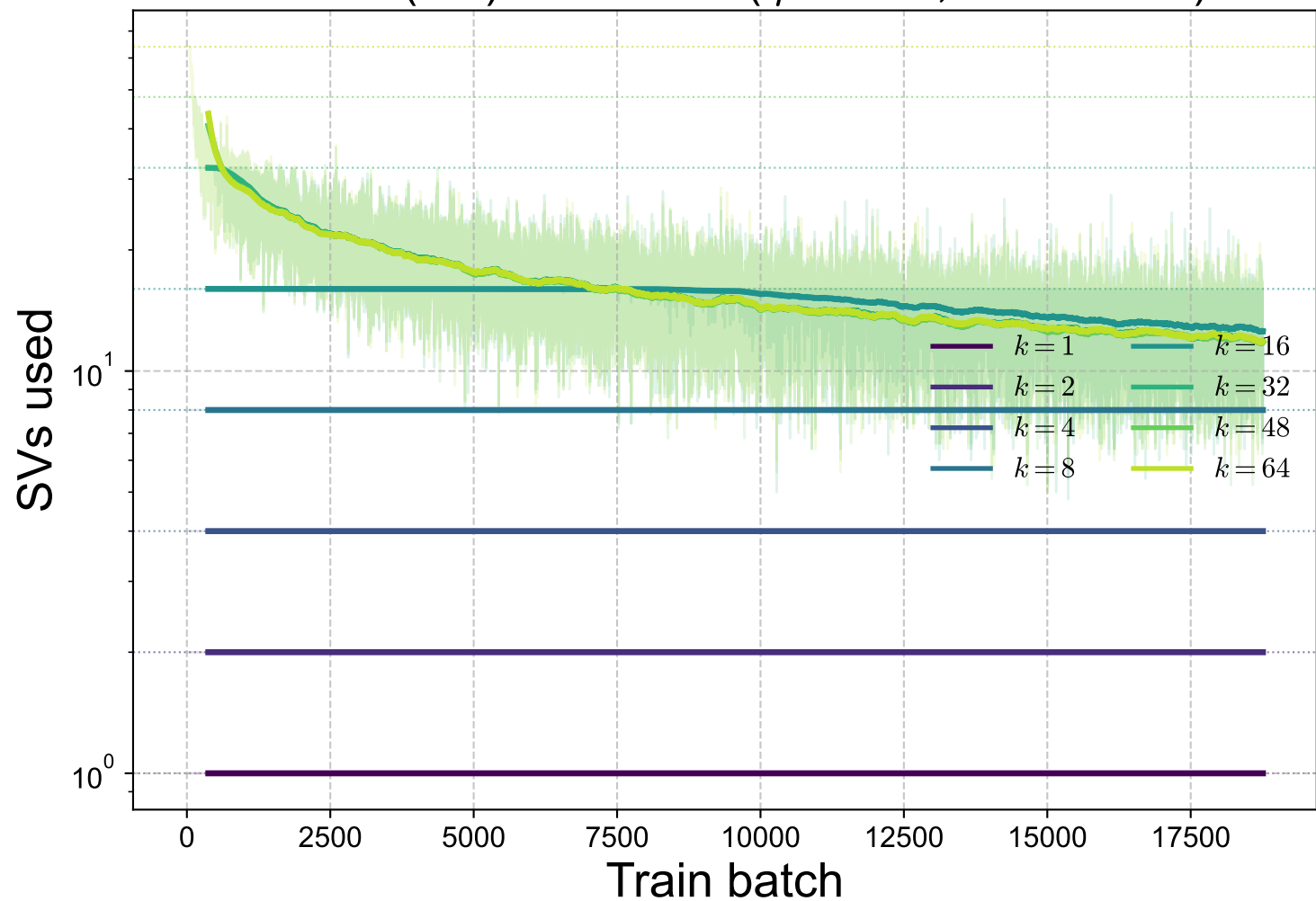
MNIST (CE): SVs used ( \eta = 10^{-1} , \text{rtol} = 10^{-3} )
