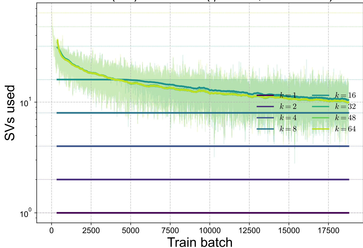
MNIST (CE): SVs used ( \eta = 10^{-1} , \text{rtol} = 10^{-2} )
