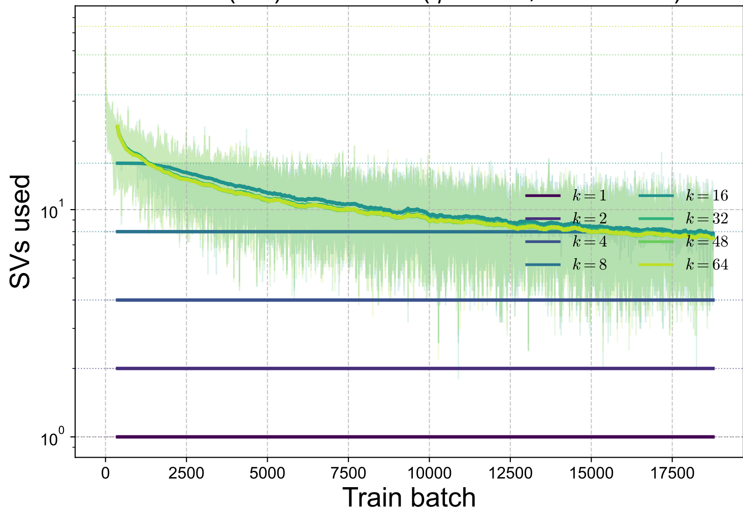
MNIST (CE): SVs used ( \eta = 10^{-1} , \text{rtol} = 10^{-1} )
