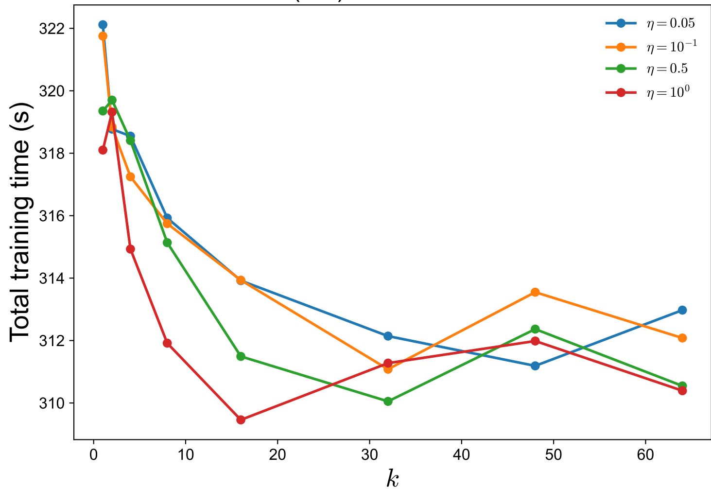
MNIST (CE): Sven wall time vs k
