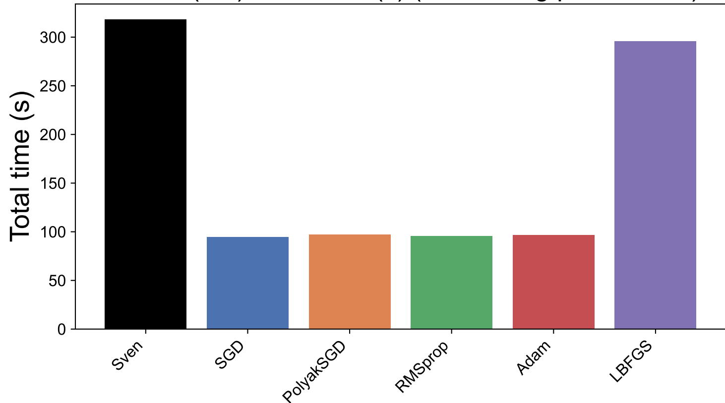
MNIST (CE): total time (s) (best config per method)
