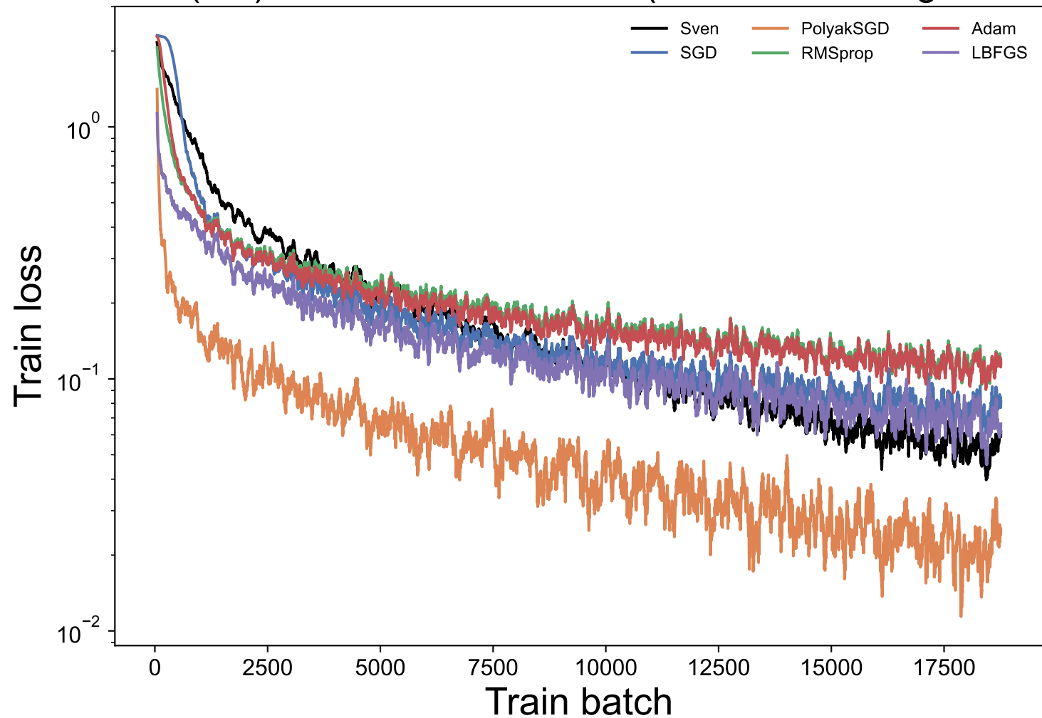
MNIST (CE): batch-level train loss (50-batch moving average)
