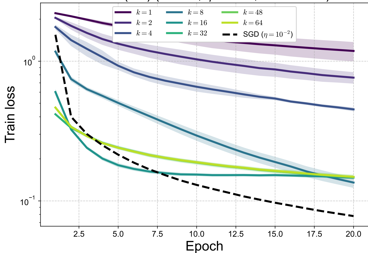
MNIST (CE) ( B = 64 , \eta = 10^{-1} , \text{rtol} = 10^{-4} )
