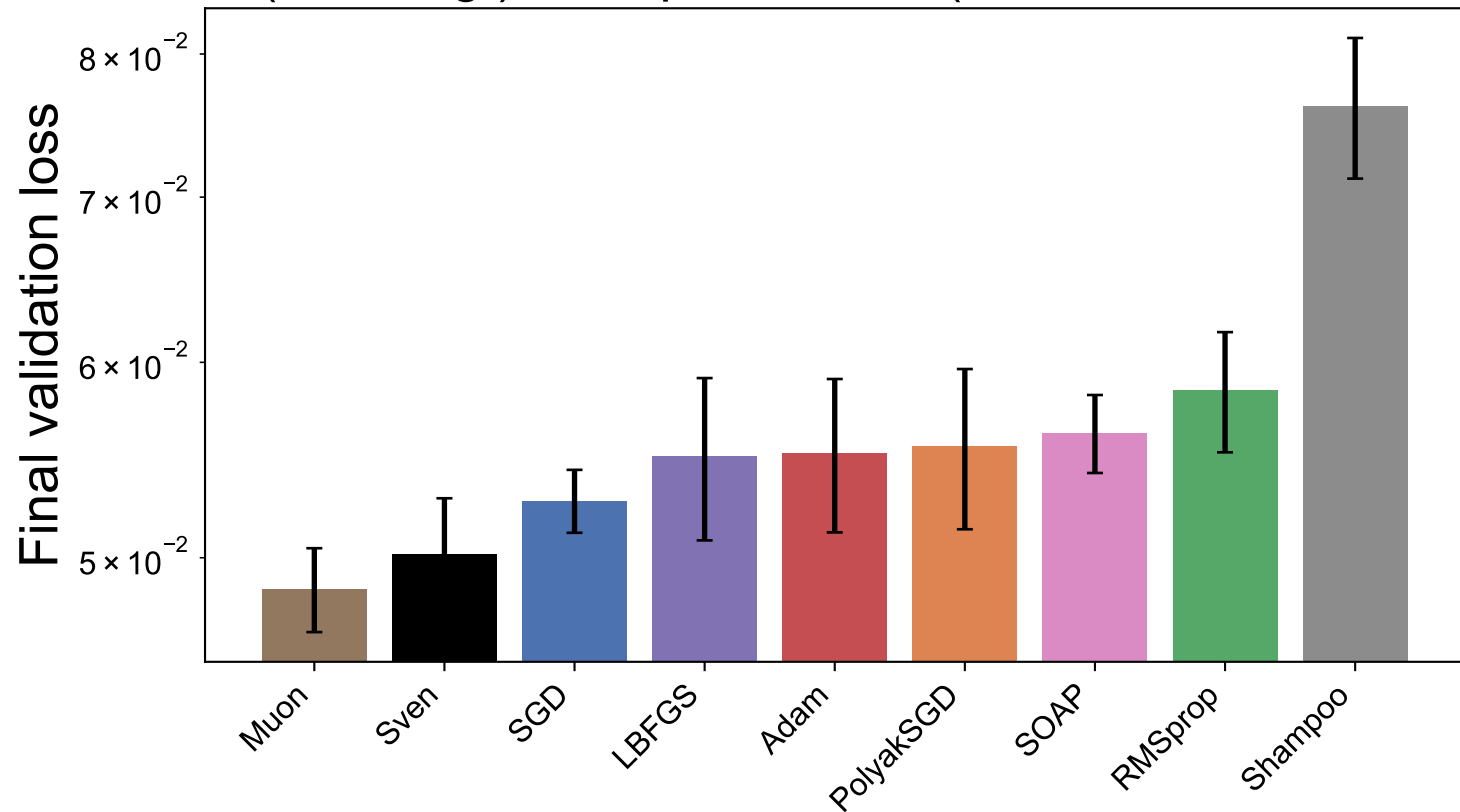
MNIST (label reg.): best per method (mean \pm s.d. over 5 seeds)
