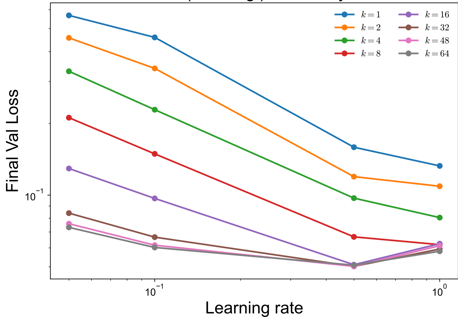
MNIST (label reg.): sensitivity to lr
