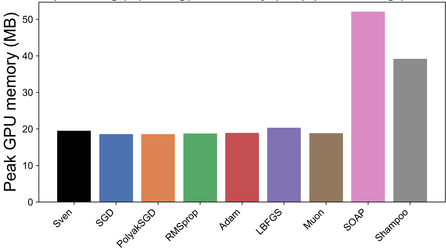
MNIST (label reg.): peak gpu memory (mb) (best config per method)
