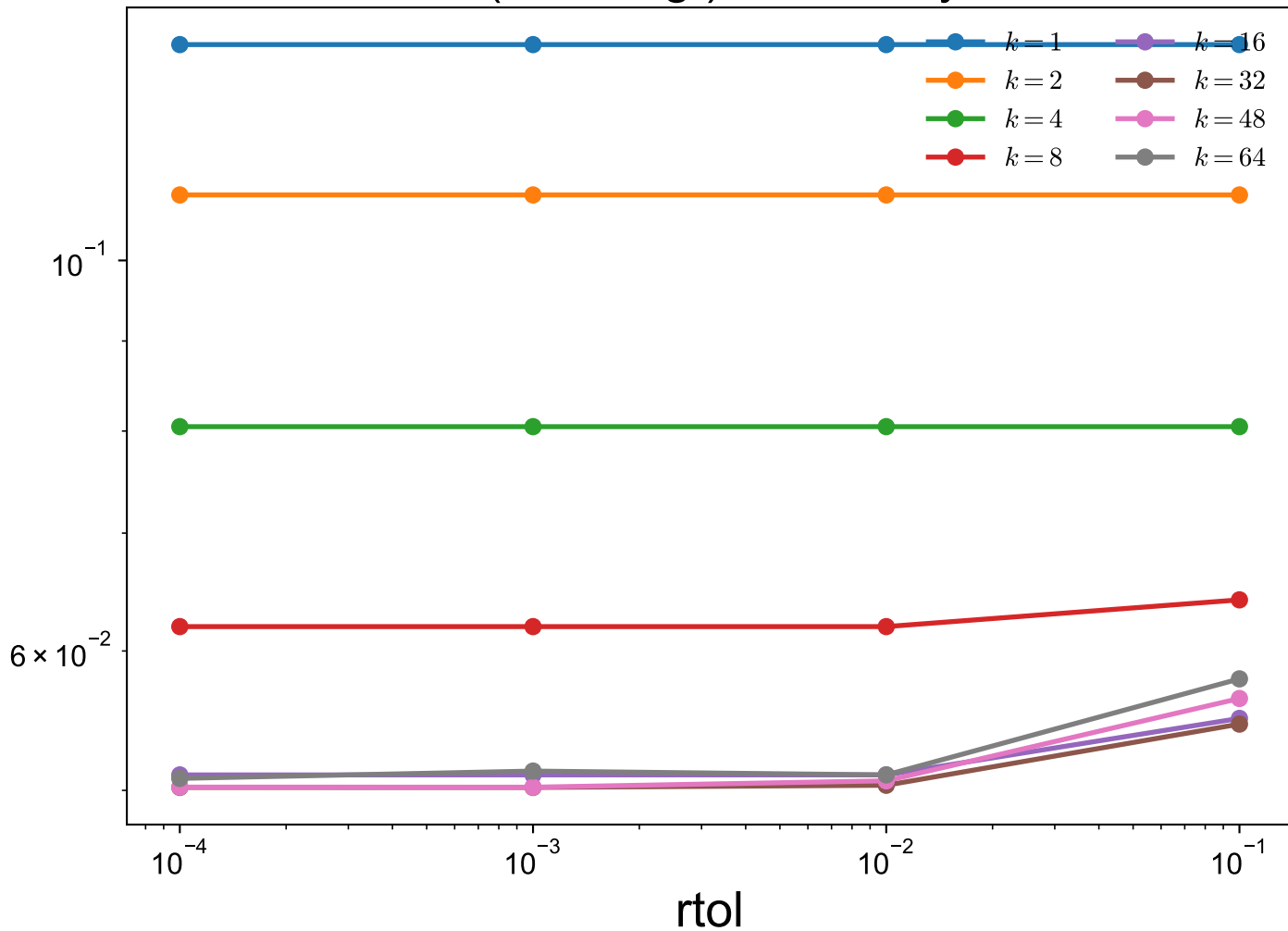
MNIST (label reg.): sensitivity to rtol
