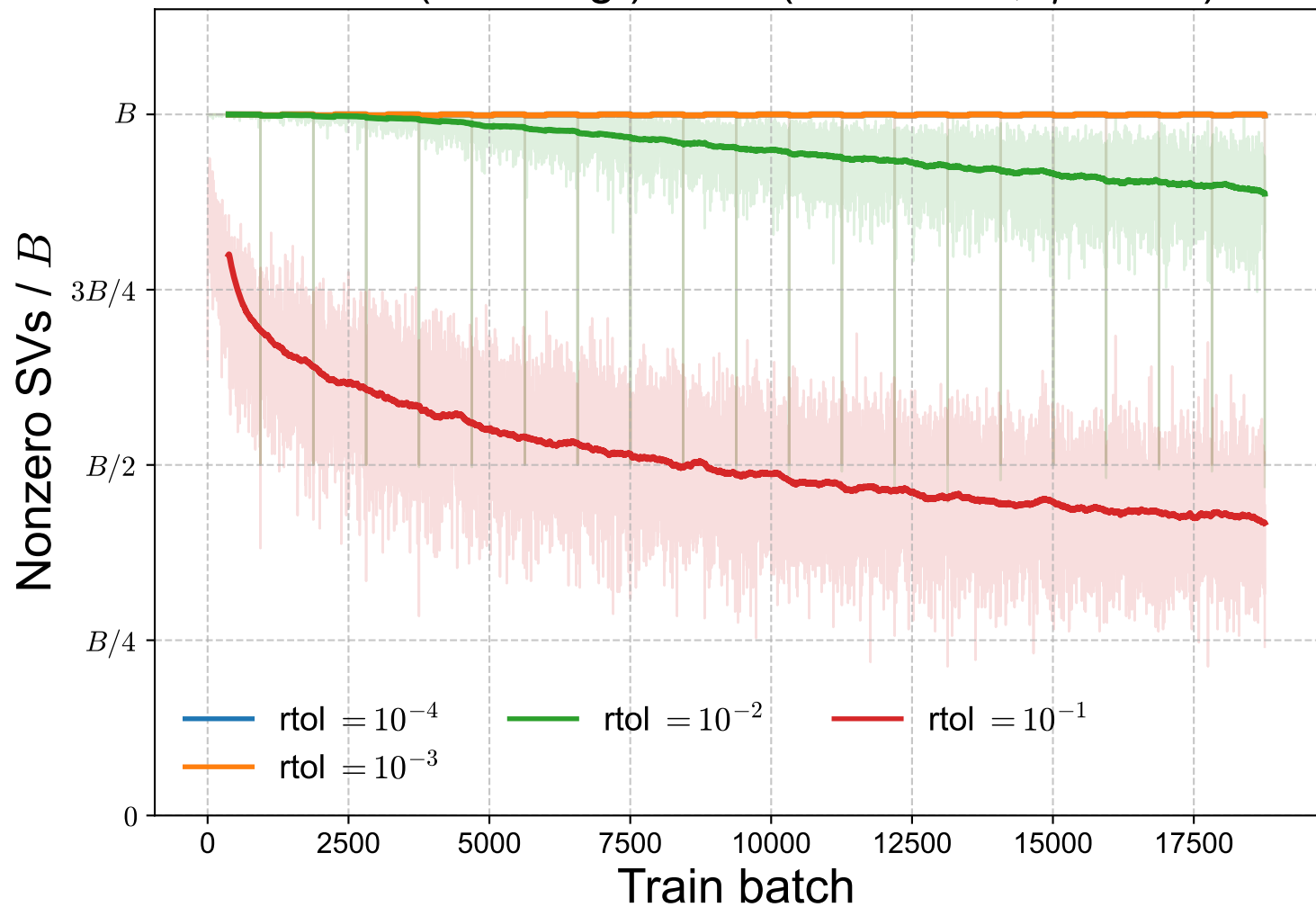
MNIST (label reg.): rank ( k = B = 64 , \eta = 0.05 )
