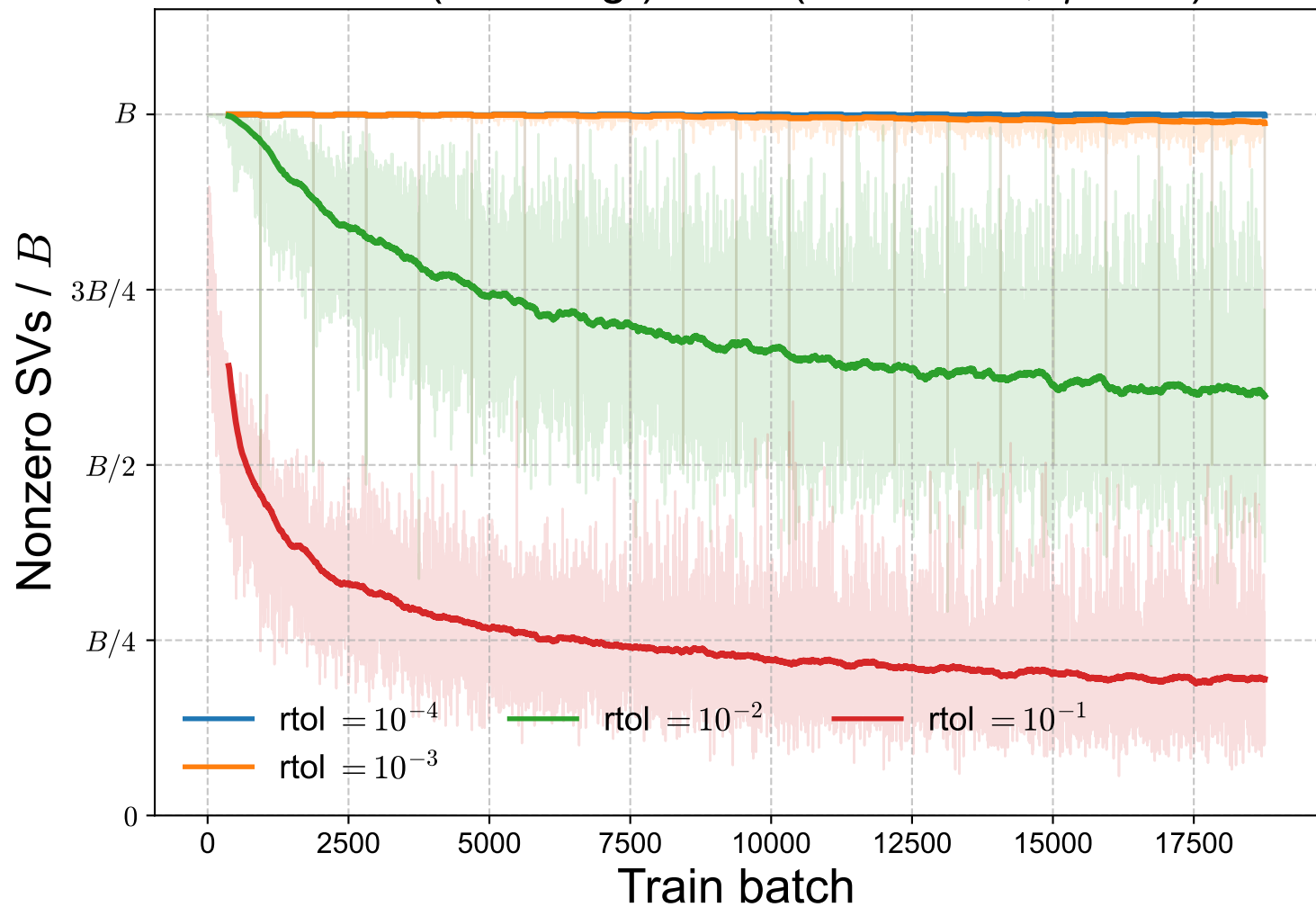
MNIST (label reg.): rank ( k = B = 64 , \eta = 0.5 )
