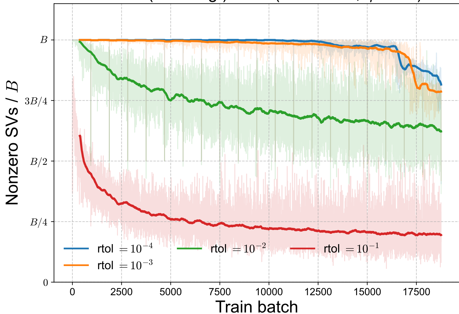
MNIST (label reg.): rank ( k = B = 64 , \eta = 10^0 )
