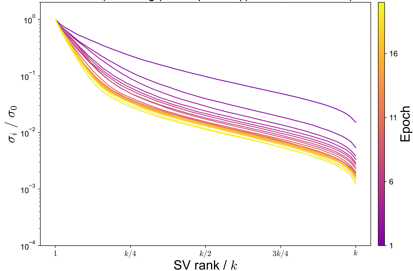
MNIST (label reg.): SV spectra ( \eta = 0.5 , \text{rtol} = 10^{-4} )
