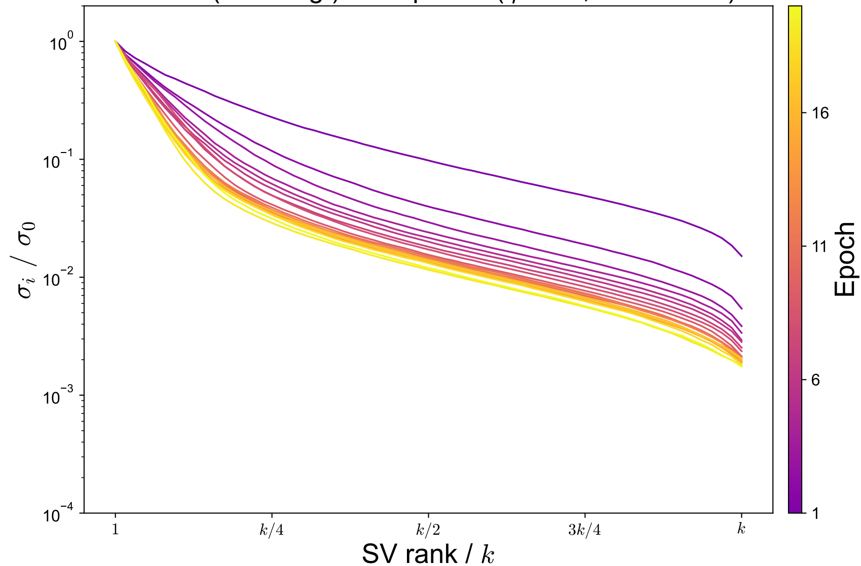
MNIST (label reg.): SV spectra ( \eta = 0.5 , \text{rtol} = 10^{-3} )
