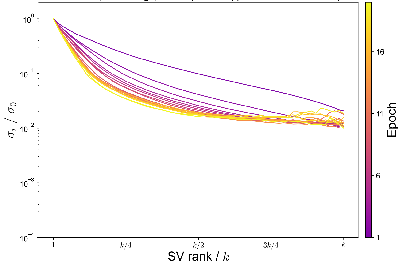
MNIST (label reg.): SV spectra ( \eta = 0.5 , \text{rtol} = 10^{-2} )
