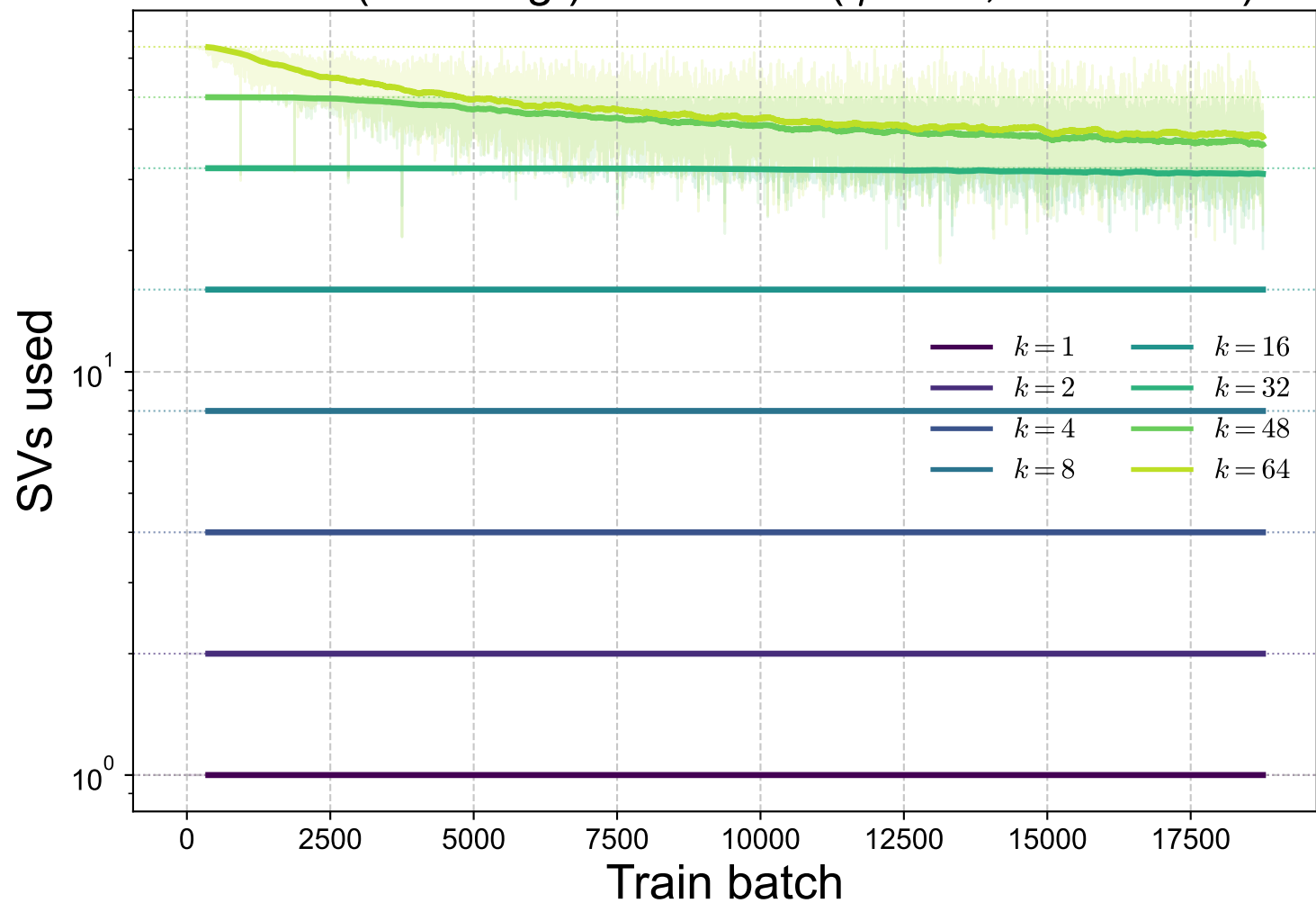
MNIST (label reg.): SVs used ( \eta = 0.5 , \text{rtol} = 10^{-2} )
