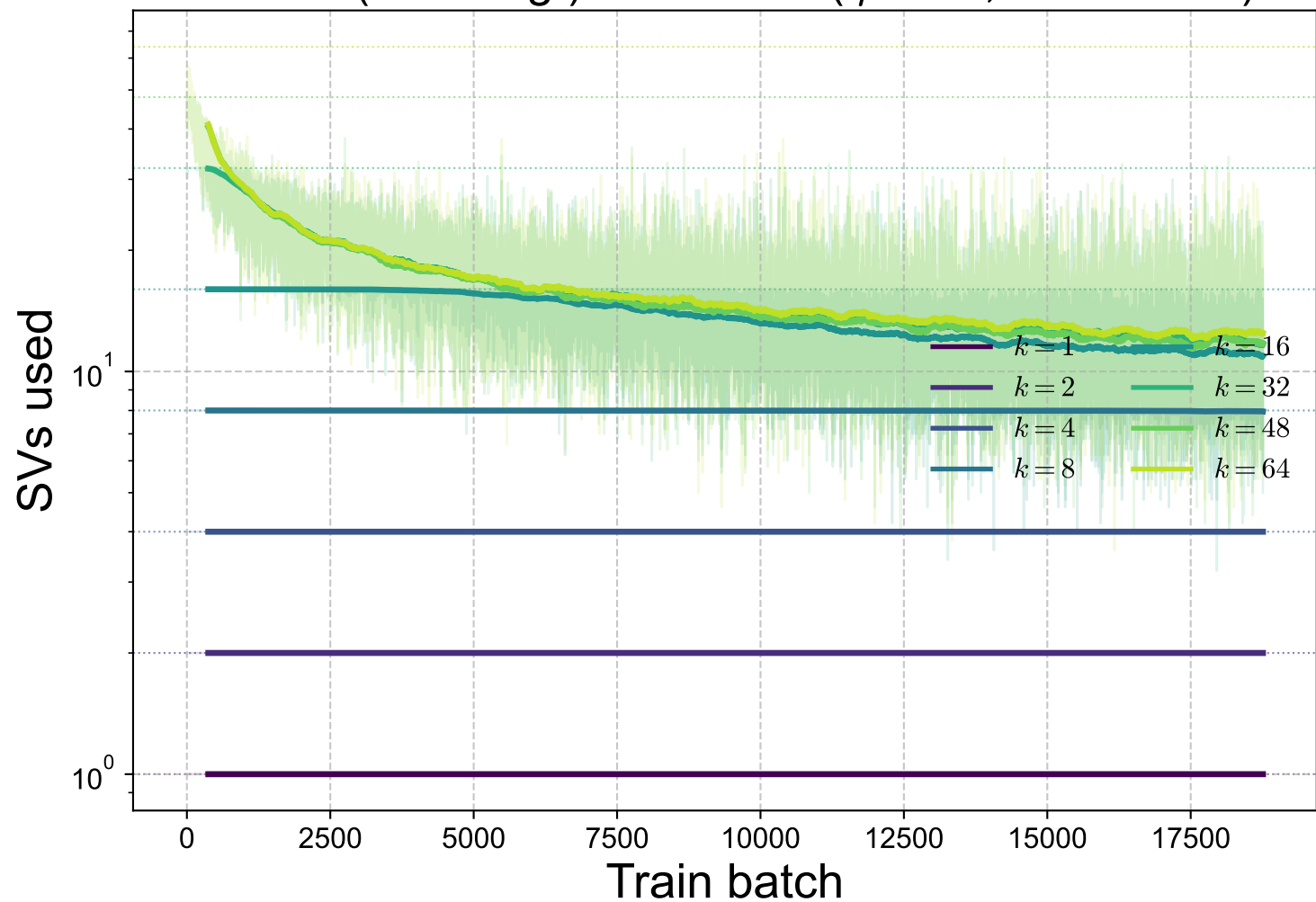
MNIST (label reg.): SVs used ( \eta = 0.5 , \text{rtol} = 10^{-1} )
