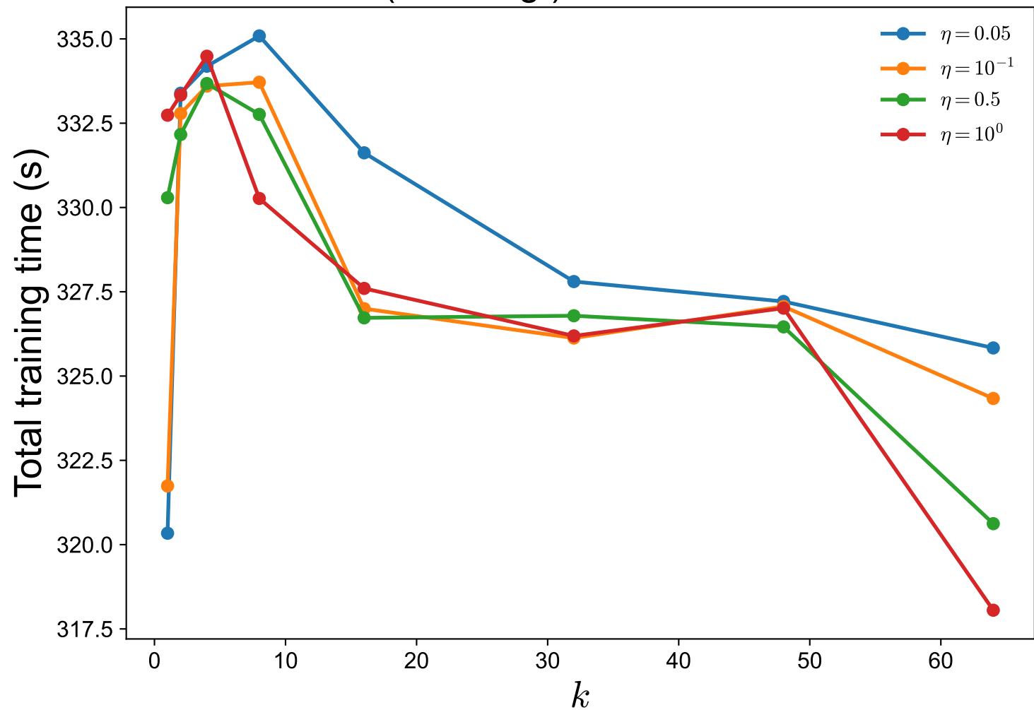
MNIST (label reg.): Sven wall time vs k
