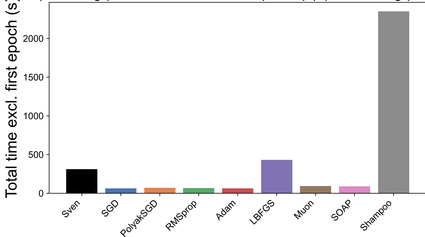
MNIST (label reg.): total time excl. first epoch (s) (best config per method)
