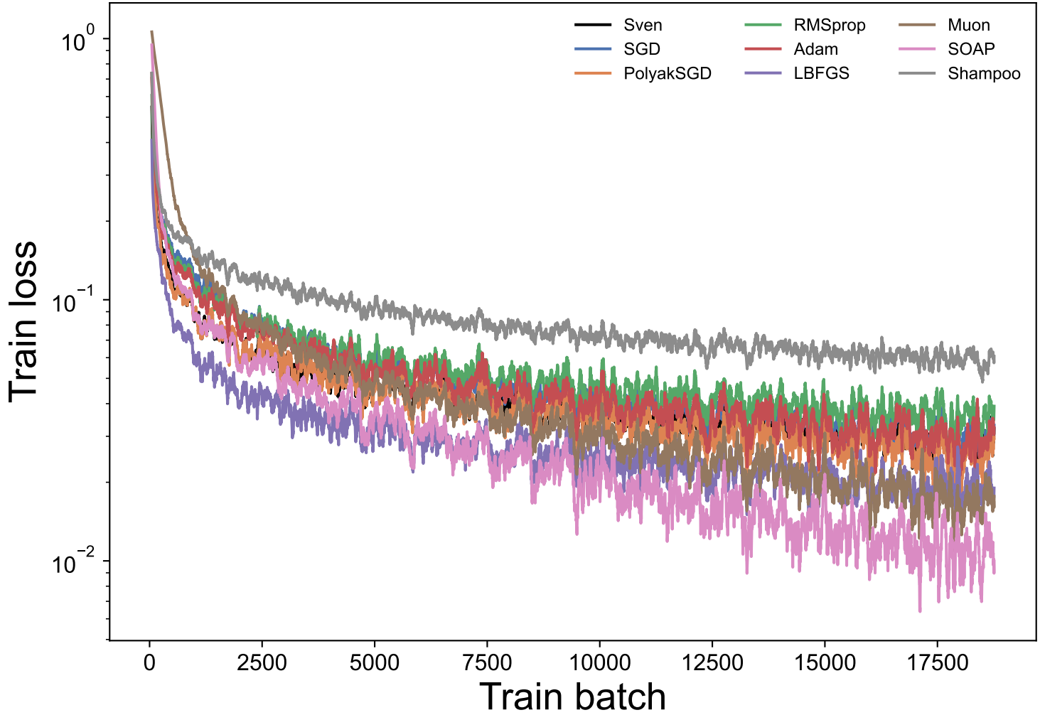
MNIST (label reg.): batch-level train loss (50-batch moving average)
