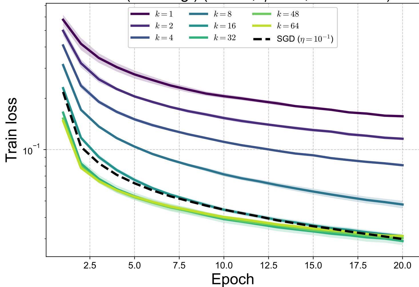
MNIST (label reg.) ( B = 64 , \eta = 0.5 , \text{rtol} = 10^{-3} )
