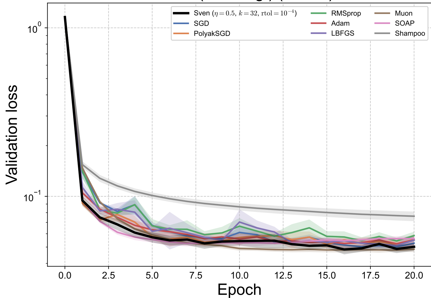
MNIST (label reg.) ( B = 64 )
