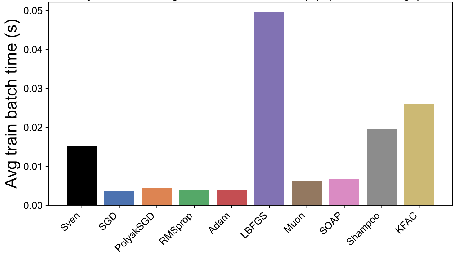
Random Polynomial: avg train batch time (s) (best config per method)
