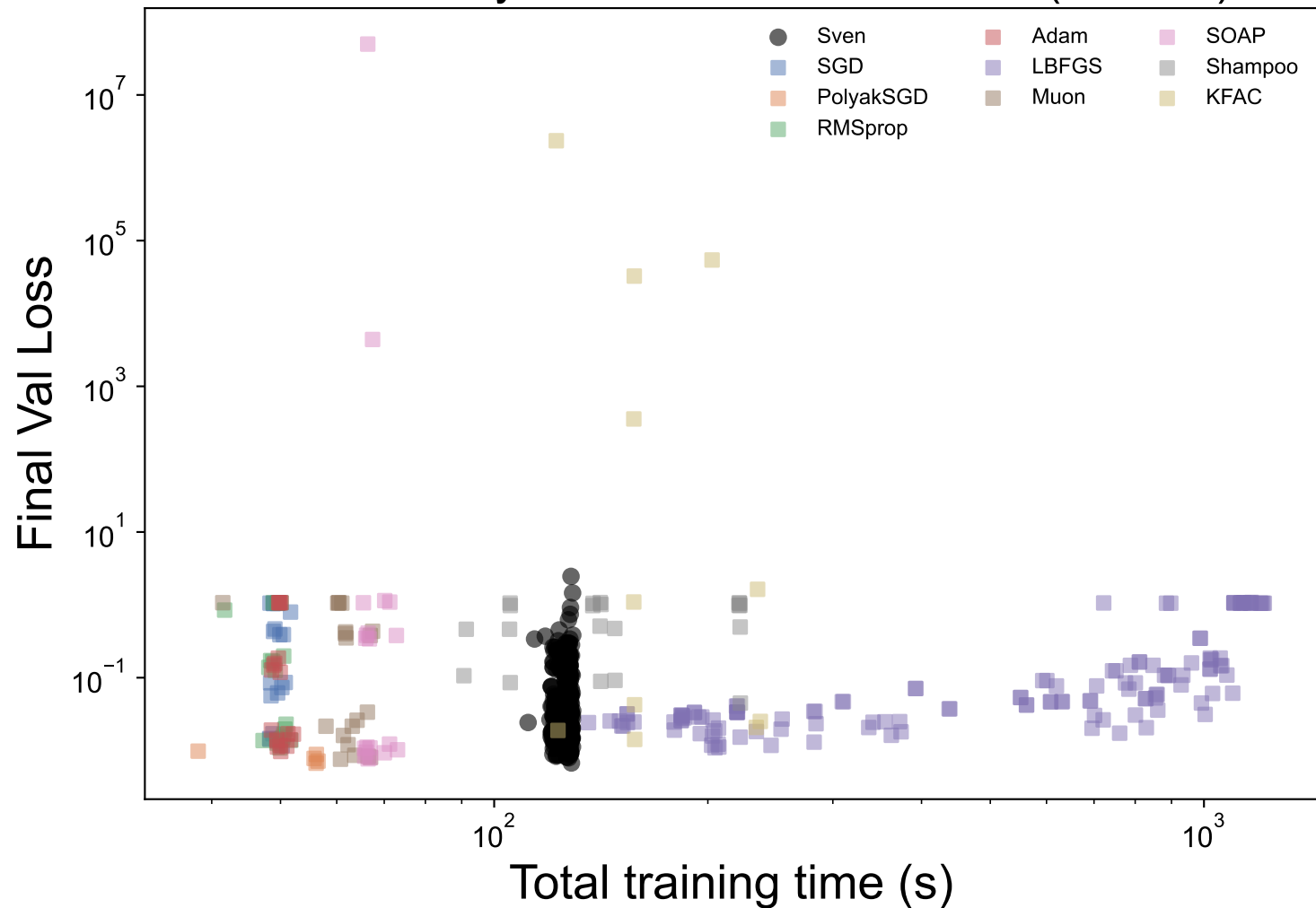
Random Polynomial: loss vs wall time (all runs)
