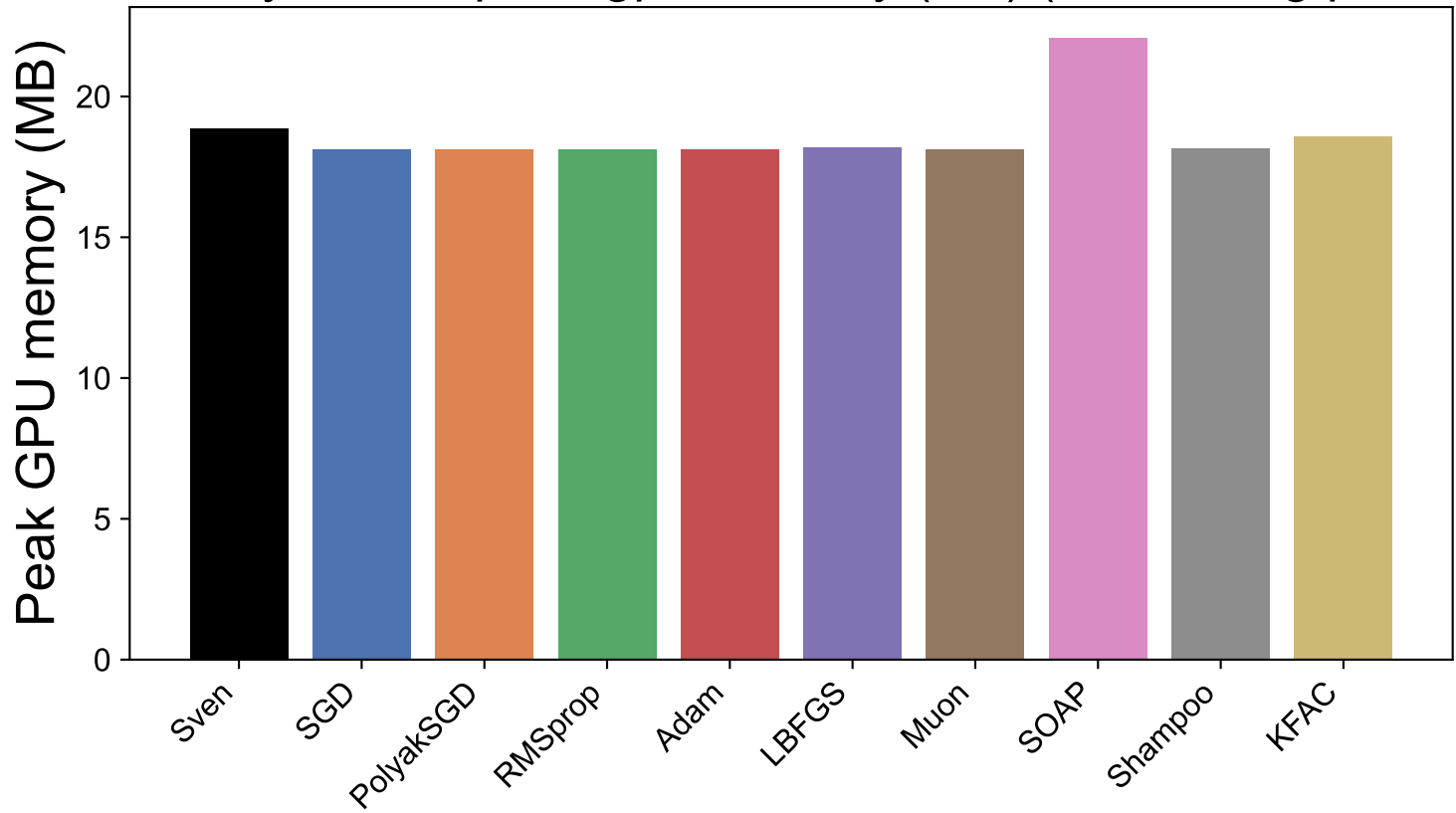
Random Polynomial: peak gpu memory (mb) (best config per method)
