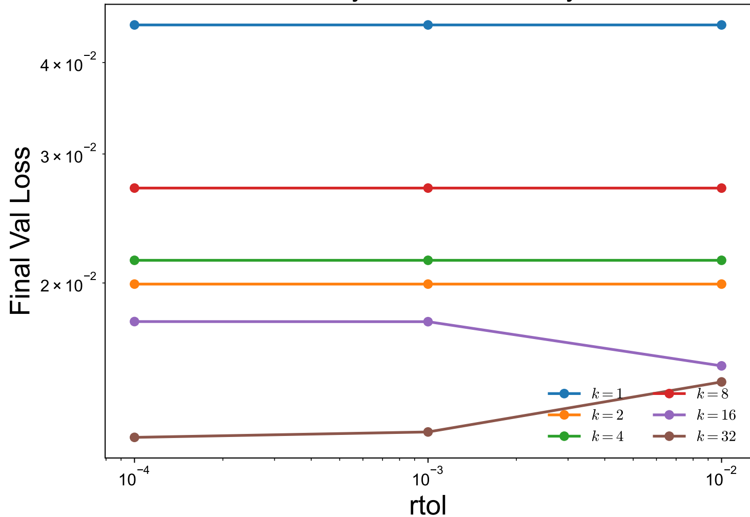
Random Polynomial: sensitivity to rtol
